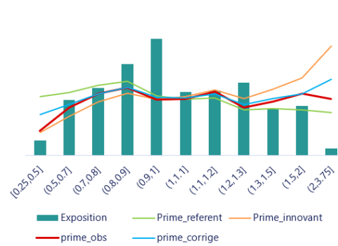
FIGURE 28 – Representation of technical premium corrected
