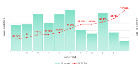
FIGURE 21 – Curve of multiplicative factors of the modalities of the traditional risk zoning
